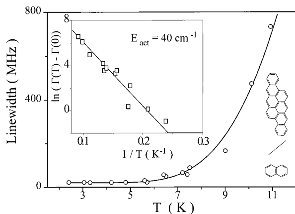
Figure 9. Dependence of the line width of a single dibenzanthanthrene molecule in a naphthalene crystal with temperature. The data are well fit by an Arrhenius plot. The activation energy corresponds to a local mode in the fluorescence spectrum.
